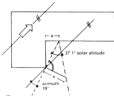
4 Plan
